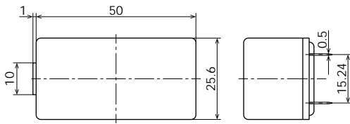
External dimensions
