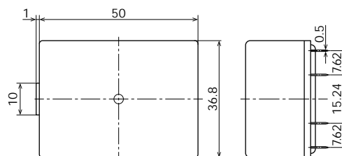
External dimensions
