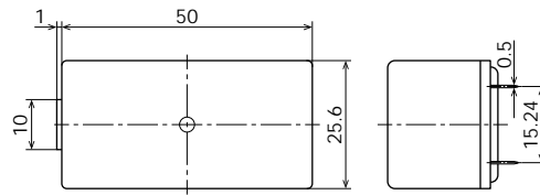
External dimensions
