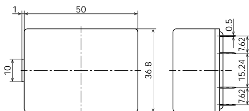
External dimensions
