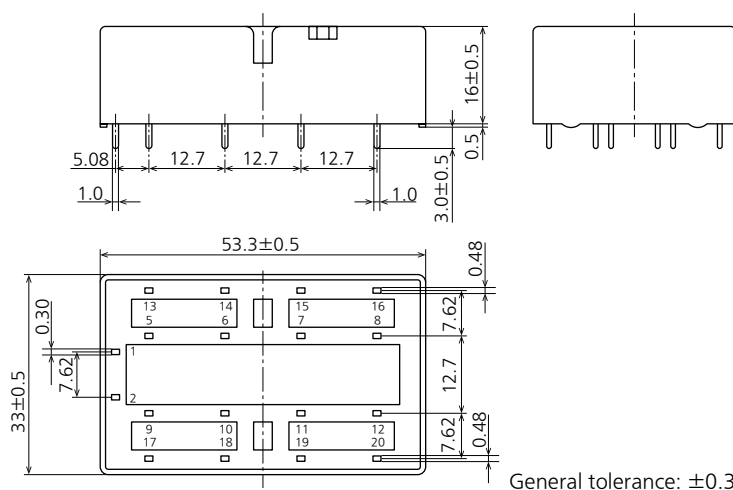
External dimensions
