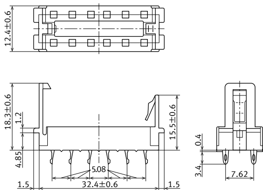
External dimensions
