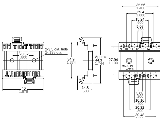
External dimensions
