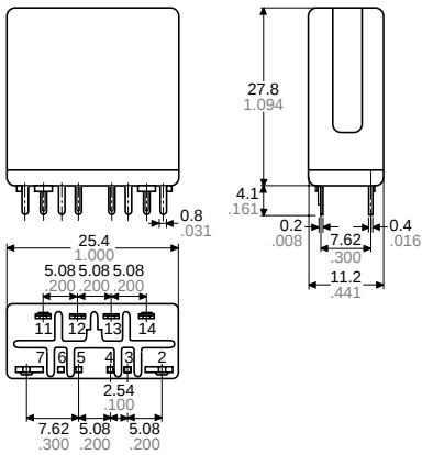
External dimensions
