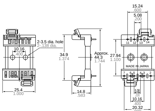
External dimensions
