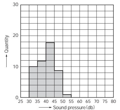
When release (At contact breaking)
