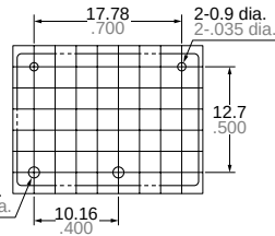
PC board pattern (Copper-side view)
