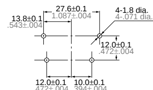
(Copper-side view)
