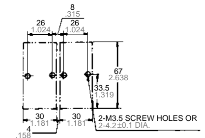
Layout for tandem mounting
