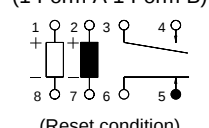
(Reset condition)
