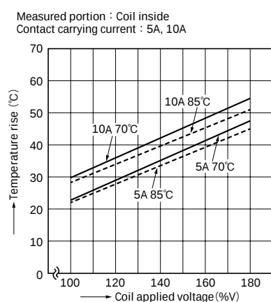
3-1. Coil temperature characteristics (1 Form A)
