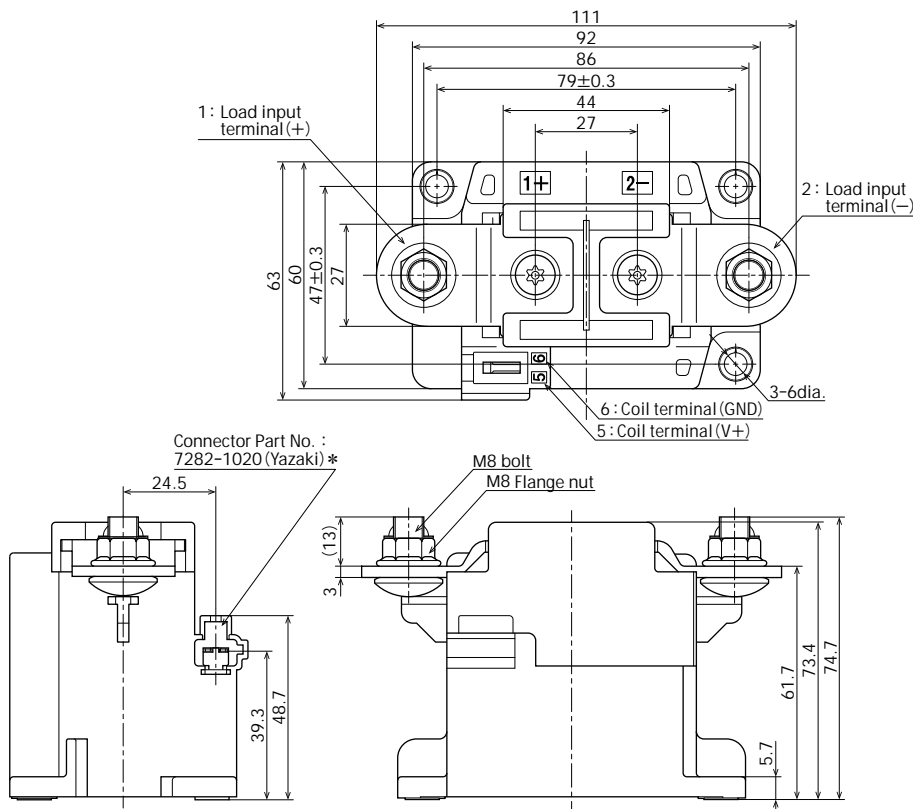
External dimensions
