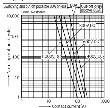
2-3. Switching and cut-off life curve (80 A type)
