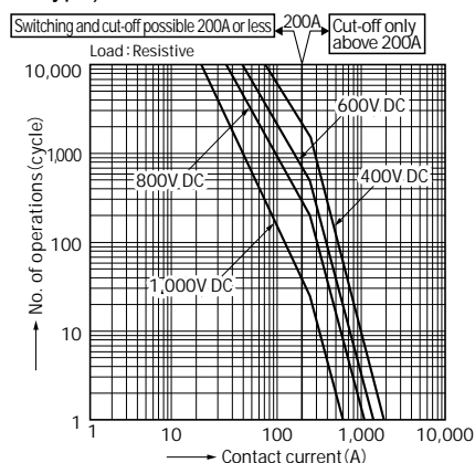
2-4. Switching and cut-off life curve (200 A type)
