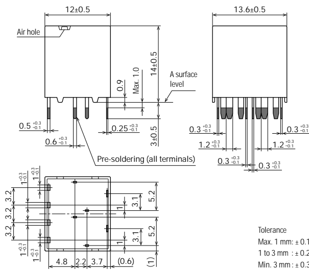
External dimensions
