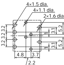
PC board pattern (BOTTOM VIEW)
