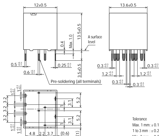
External dimensions
