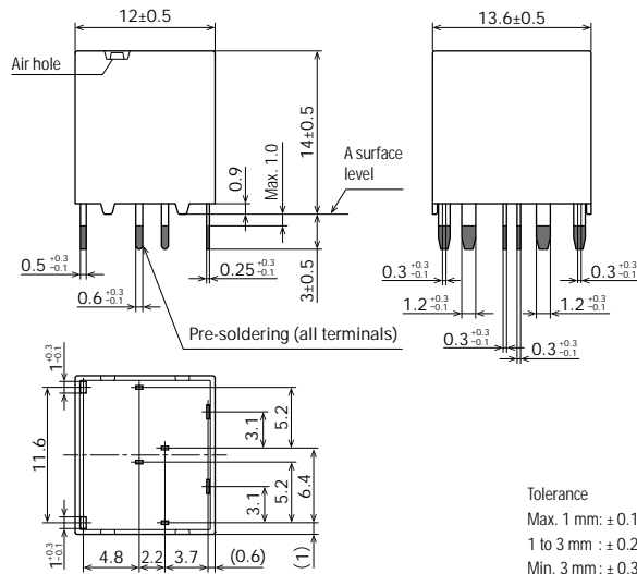
External dimensions
