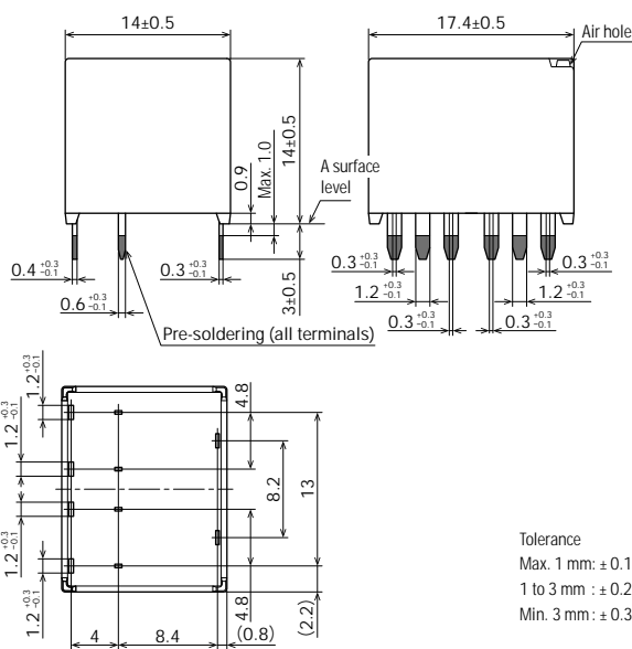
External dimensions
