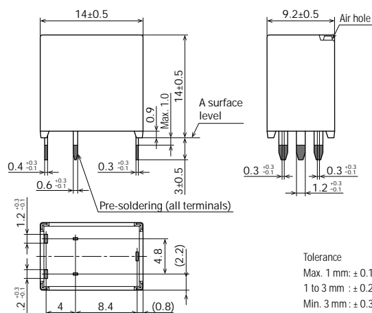
External dimensions
