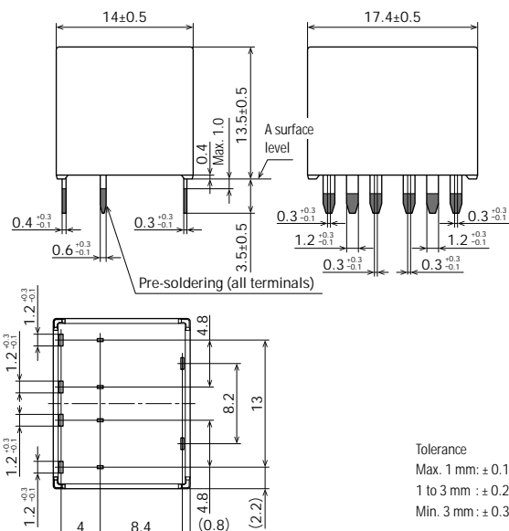
External dimensions
