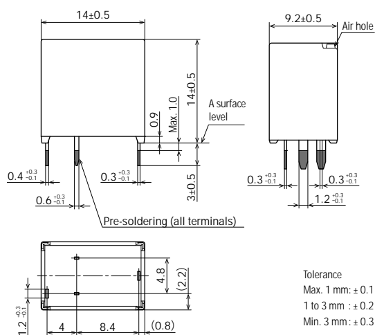
External dimensions
