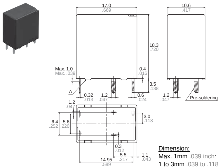
External dimensions
