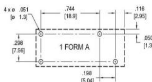
VIEWED TOWARD TERMINALS
