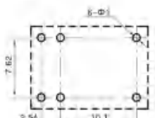
Mounting hole size (bottom view) 安装孔尺寸 (底视图)
