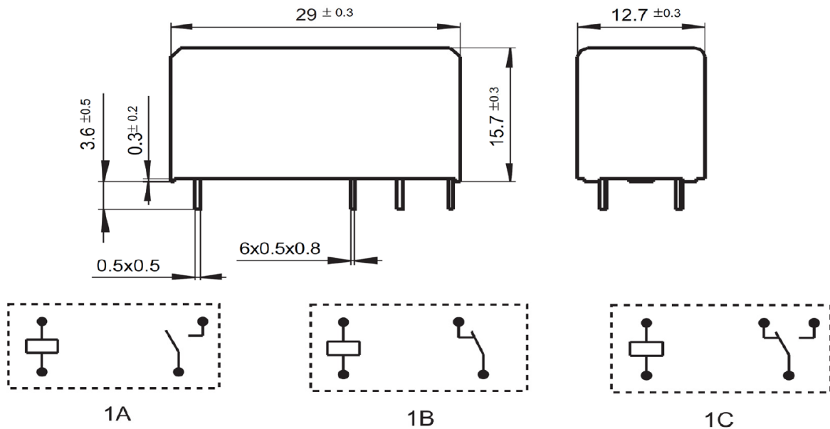
接线图 (底视图) Wiring Diagram (bottom view)
