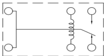
接线图 (底视图) Wiring Diagram bottom view
