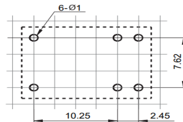
P.C.B.Lavout (bottom view)
