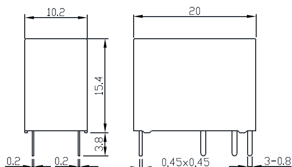
Outline Dimensions
