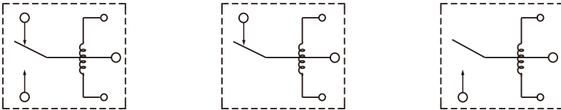
Wiring diagram (bottom view) 接线图 (底视图)
